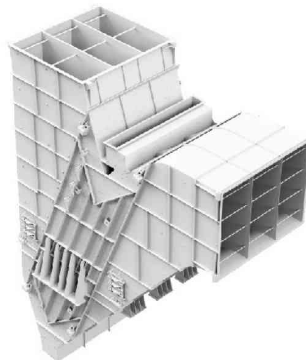
Separators
