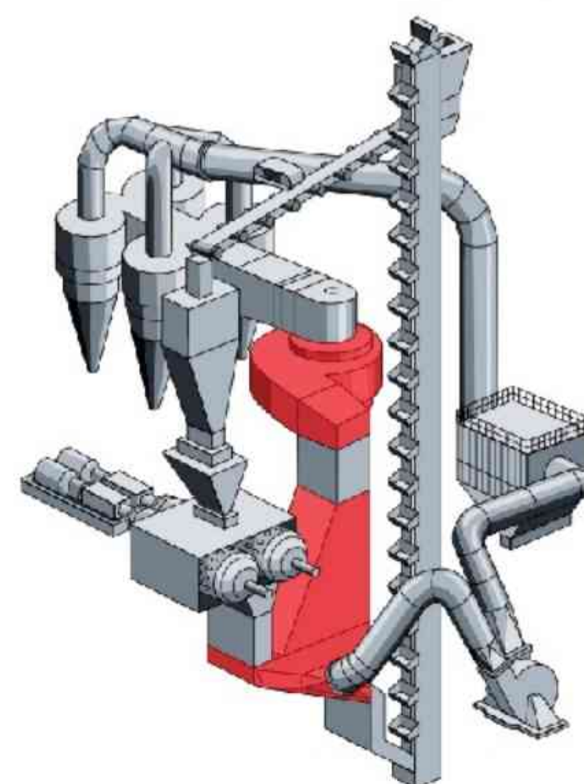
Separators
