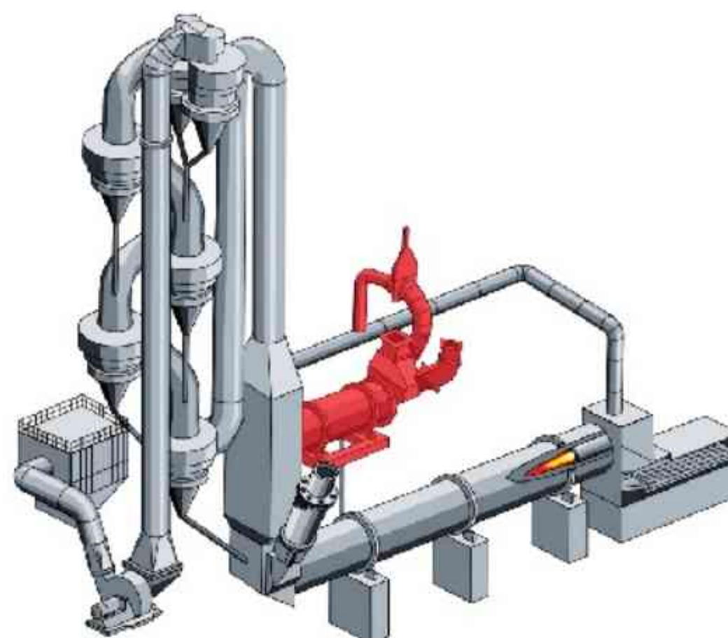
Pyrorotor
